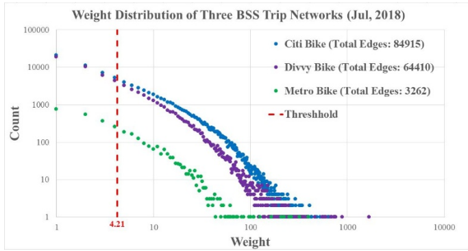
FIGURE 3: WEIGHT DISTRIBUTION EXAMPLES OF THREE TRIP NETWORKS (JUL, 2018)
