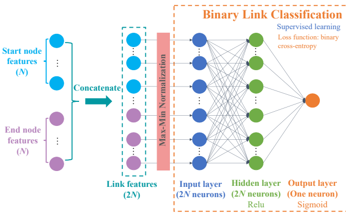
FIGURE 4: Architecture of the ANN link predicting model.
