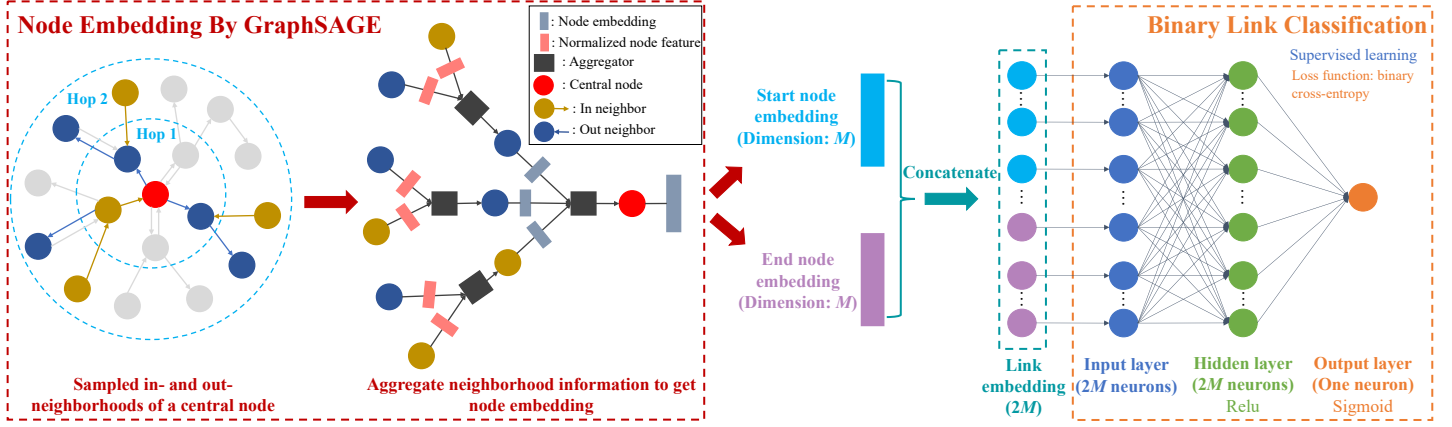
FIGURE 5: Architecture of the GraphSAGE link predicting model.
